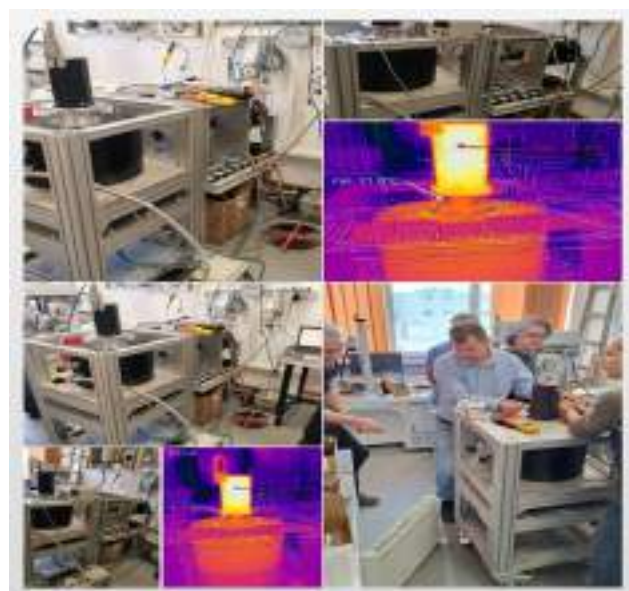
Fig. Testing and validation of the Disep prototype (TRL6)
