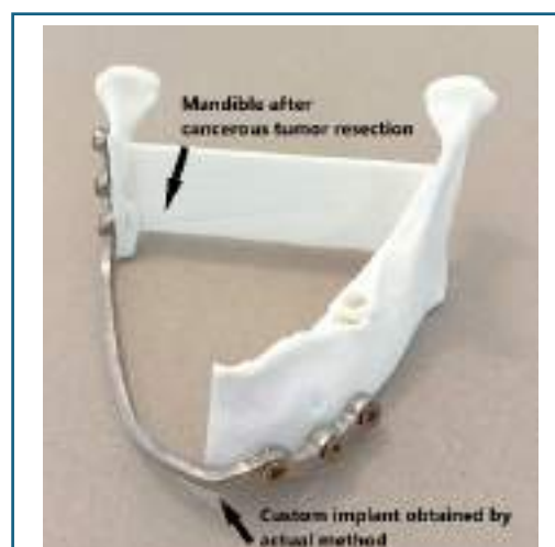
Fig. 1. Mandibular reconstruction developed using Ti-Gr composite and manufactured through the SLM process.
