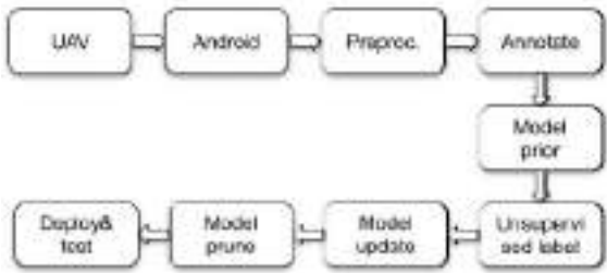
Processing pipeline
