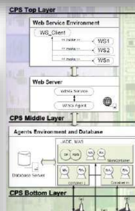
CPS 3 Layers Based Architecture
