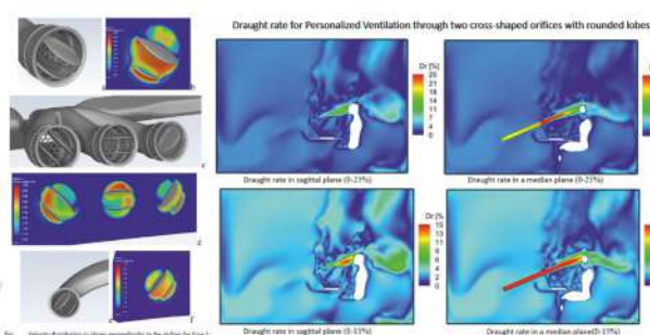
Fig. 1. Velocity distribution in plane perpendicular to the orifice for two 15% Right and 15% Left. (a) Right and 15% Left velocity distribution. (b) Down and 15% Right and 15% Left velocity distribution. (c) Left and 15% Right and 15% Left velocity distribution. (d) Left and 15% Right and 15% Left velocity distribution.
