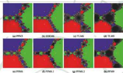
Figure 3. Basins of attraction for P_3(x)
